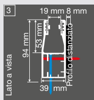
Guida unica (optional) 94 x 39 mm
